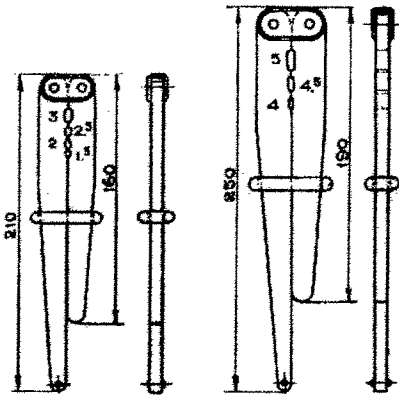
Fig 77. Wringtang.
